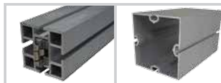
Maximax 40mm profile Maximax 80mm profile
